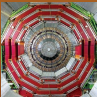
CMS
